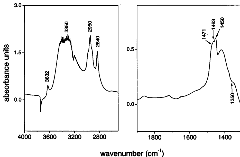
Figure 3. Infrared difference spectrum of TS-1 loaded with 4 Torr of CH 3 OH and 221 Torr of CO at 173 K.
