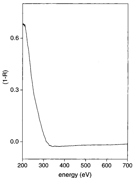
Figure 1. UV-vis reflectance spectrum of TS-1 calcined at 823 K. R = reflectance, BaSO 4 as the reference.
