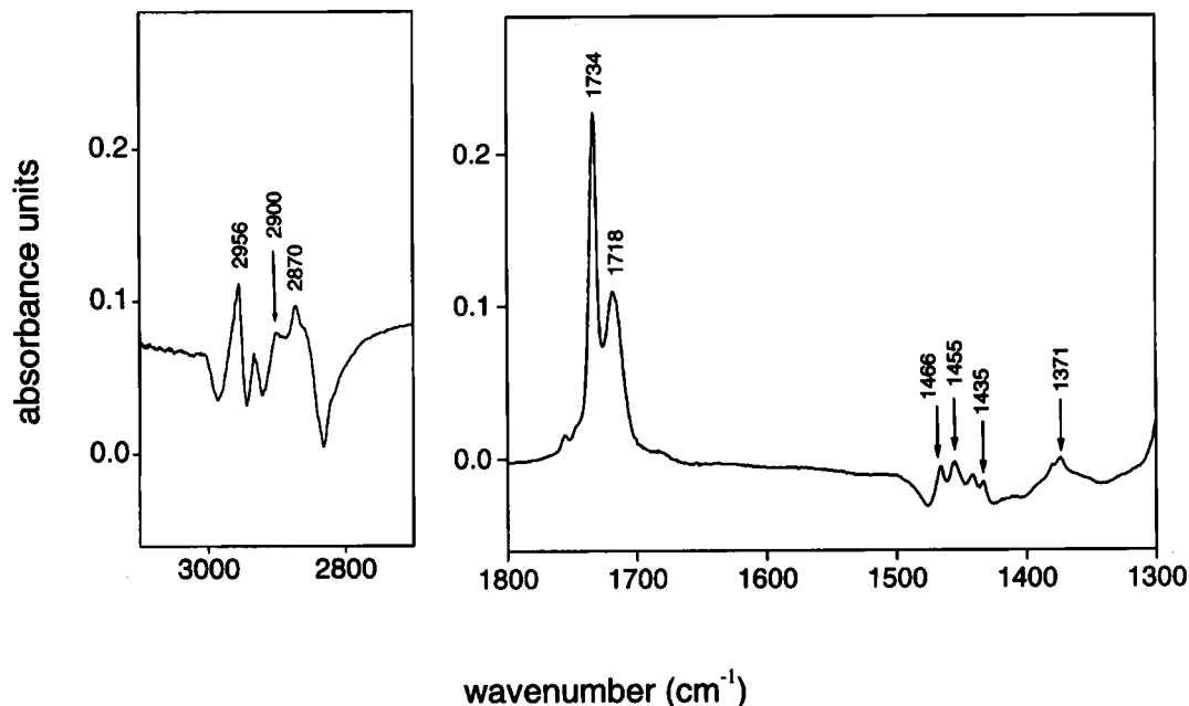
Figure 4. Infrared difference spectrum after 266-nm irradiation at 200 mW cm -2 for 3.5 h.
