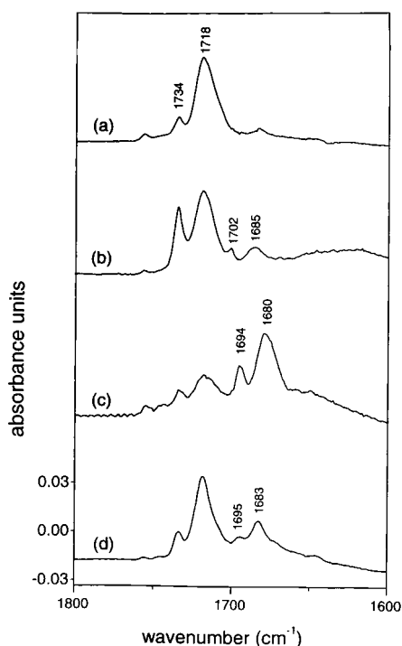
Figure 6. Photoinduced reaction of carbon monoxide and methanol in TS-1 at 173 K. Shown are the infrared difference spectra upon 266-nm irradiation for 2 h at 100\text{ mW cm}^{-2} of (a) \text{CO} + \text{CH}_3\text{OH} , (b) \text{C}^{18}\text{O} + \text{CH}_3\text{OH} , (c) \text{CO} + {}^{13}\text{CH}_3\text{OH} , (d) {}^{13}\text{CO} + \text{CH}_3\text{OH} .
