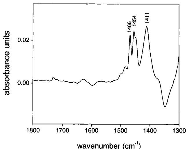
Figure 5. Infrared difference spectrum taken immediately after adsorption of 0.5 Torr of \text{CH}_2=\text{O} gas into TS-1 sieve loaded with 0.4 Torr of \text{CH}_3\text{OH} at 220 K. Bands at 1729 and 1501\text{ cm}^{-1} are due to as-yet-unreacted formaldehyde.
