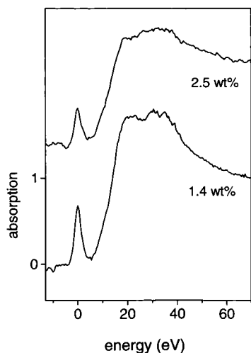
Figure 2. Ti K-edge XANES spectra of TS-1. Absorption scale is normalized to the plateau between the K-edge and the onset of the extended region.
